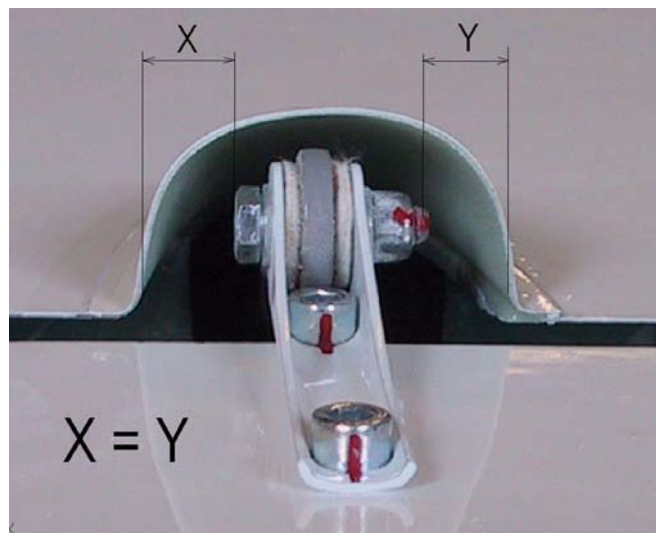
Step 10: - measurement of exact position
